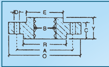
Threaded Flange
