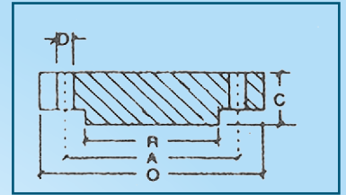
Blind Flange
