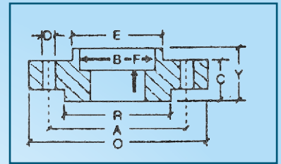
Socket-weld Flange
