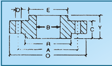
Slip-on Flange
